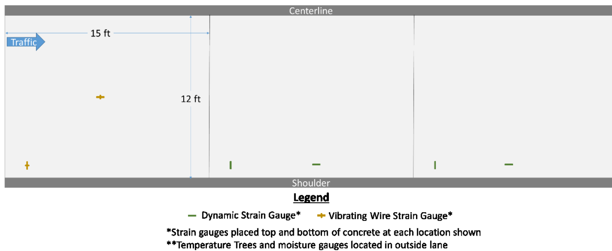
Figure 6.6 Sensor layout for Cell 238.
