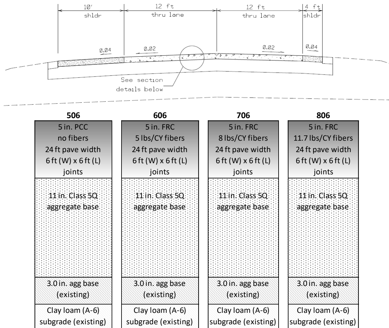
Figure 4.6 Planned section design details of FRC Cells 506 - 806.
