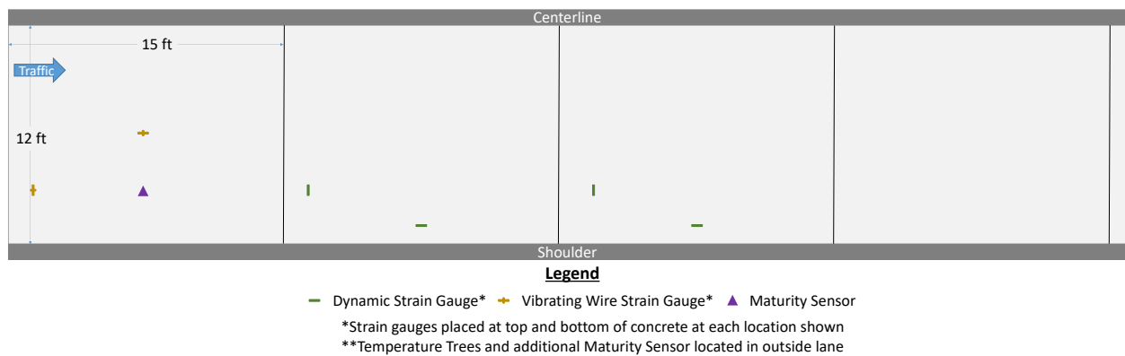
Figure 5.10 Sensor layout for Cell 324.
