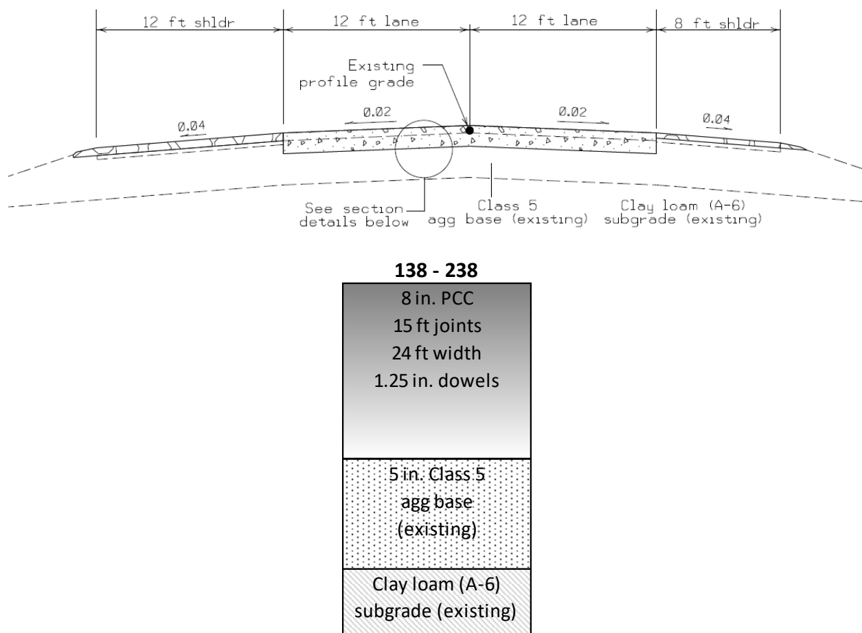
Figure 6.1 Design section details for Cells 138 and 238.
