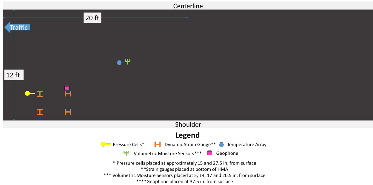
Figure 7.10 Sensor layout in Cell 186.
