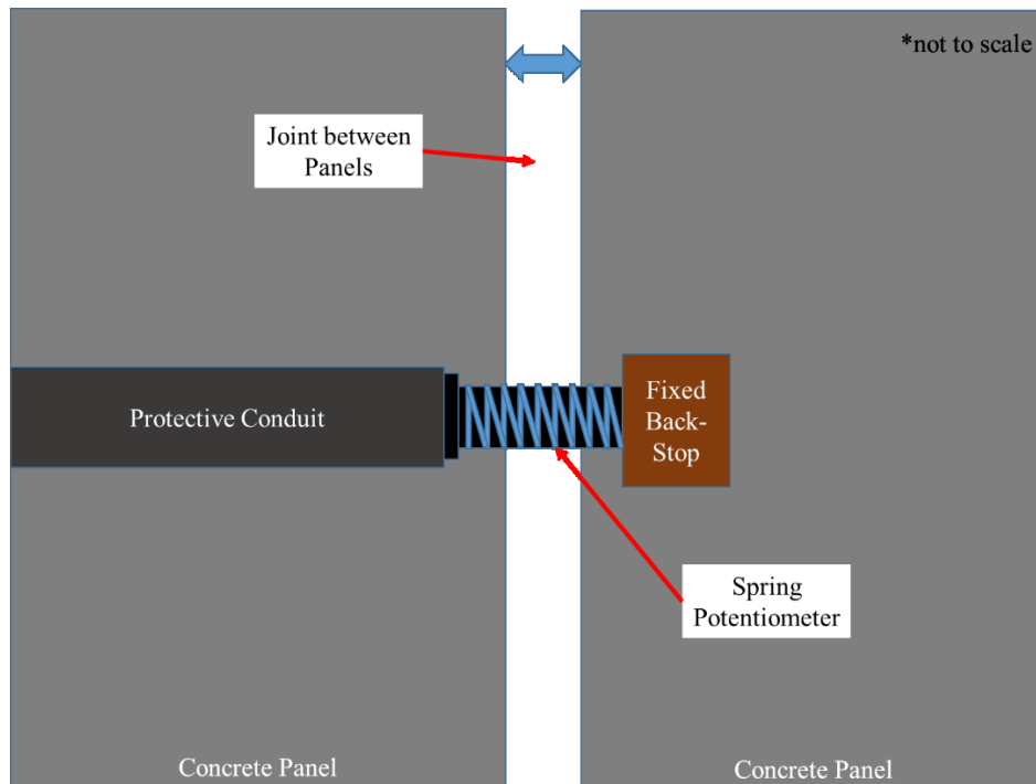
Figure 10.5 Schematic diagram of a joint opening (JO) sensor.
