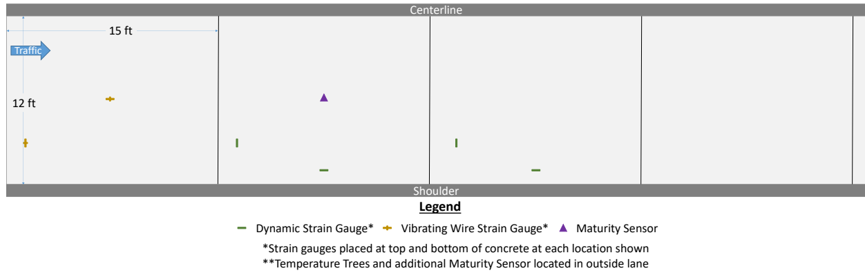
Figure 5.9 Sensor layout for Cell 224.
