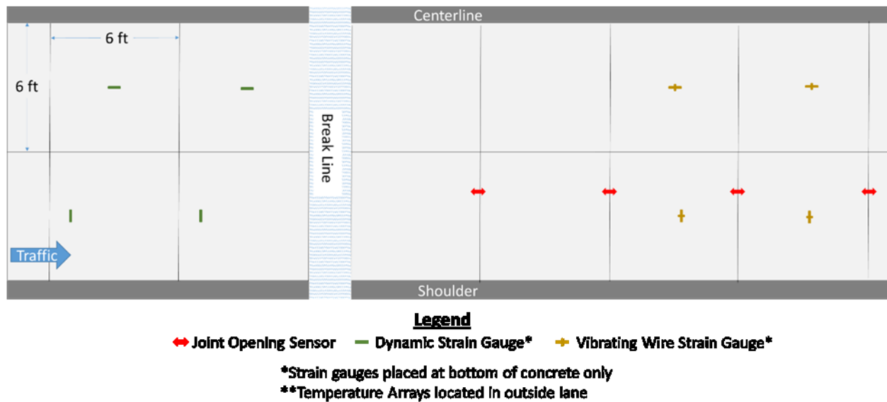
Figure 4.16 Sensor layout for FRC Cell 239.
