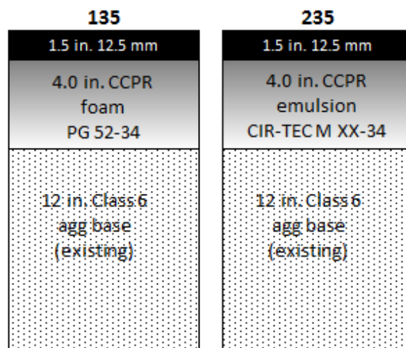
Figure 2.1 NRRA CCPR research section designs, Cells 135 and 235.
