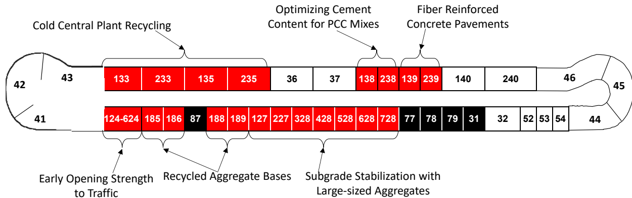
Figure 1.1 MnROAD Low Volume Road (LVR) NRRA sections.
