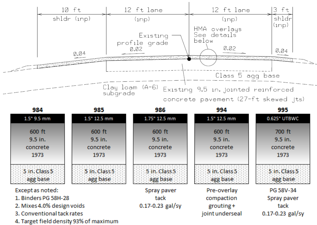
Figure 3.2 Single lift asphalt overlay section designs.
