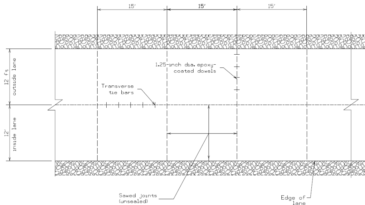
Figure 6.2 Plan detail for Cells 138 and 238.
