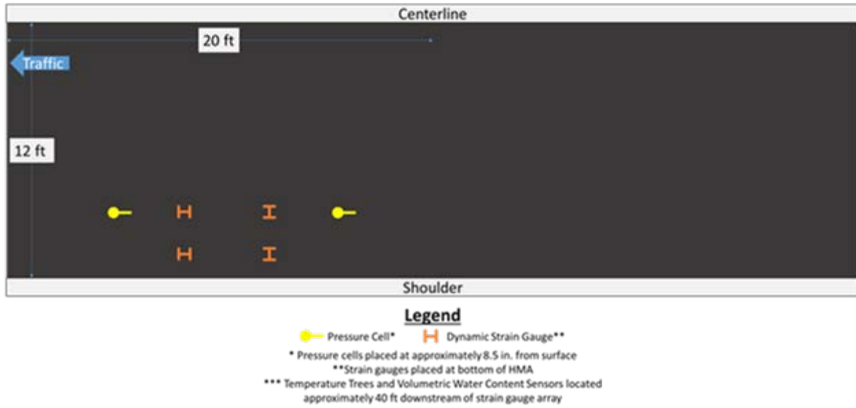
Figure 7.12 Sensor layout in Cell 728.
