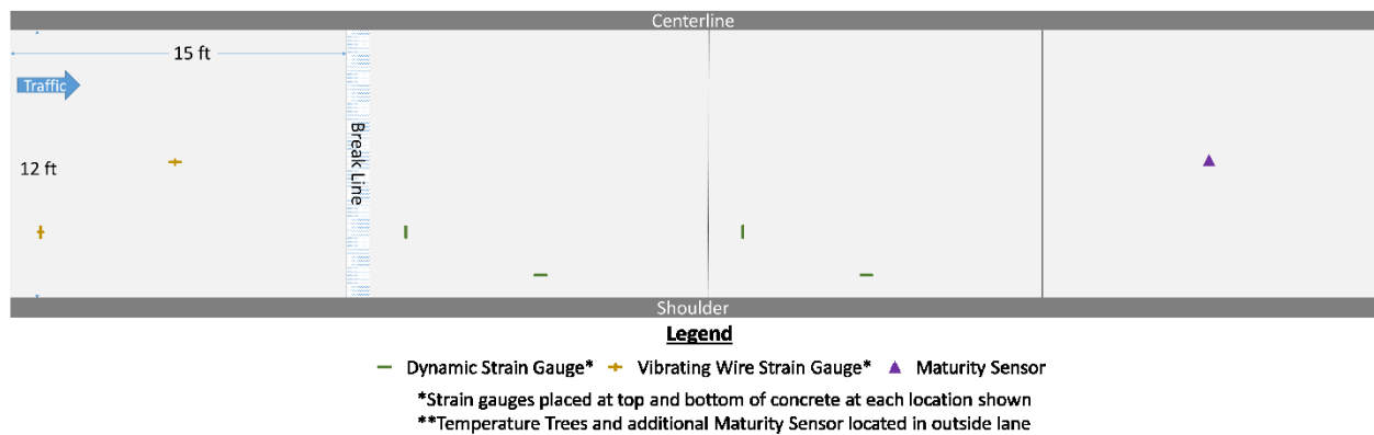
Figure 5.11 Sensor layout for Cell 424.
