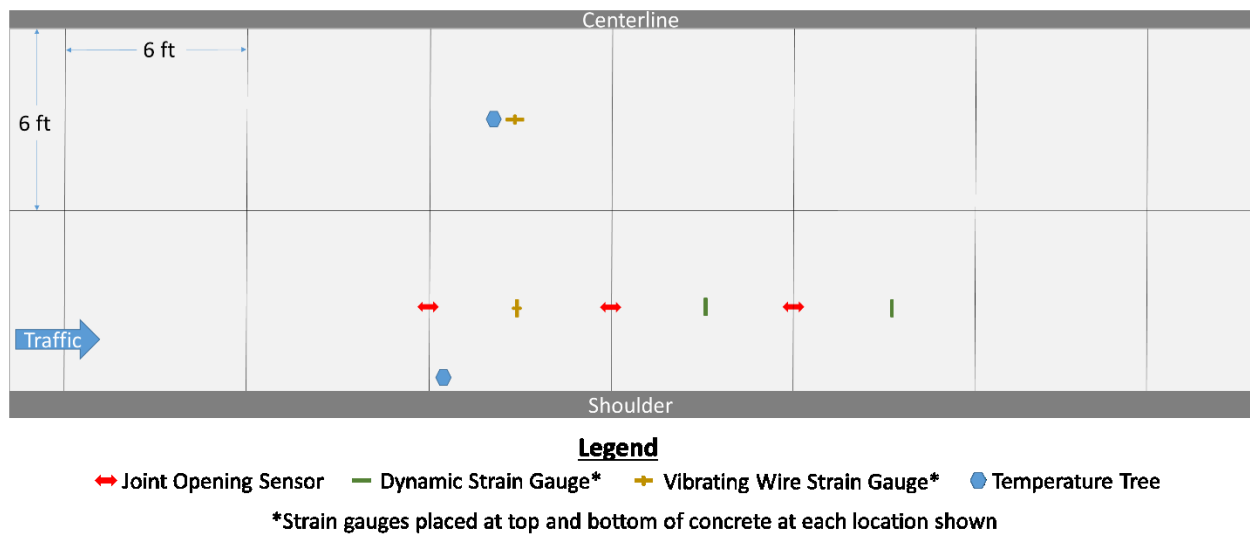
Figure 4.20 Sensor layout for FRC Cell 606.
