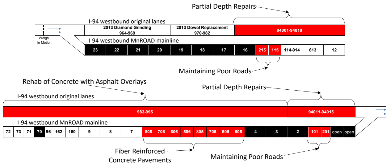
Figure 1.2 MnROAD I-94 WB (original and mainline) NRRA sections.
