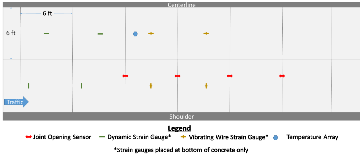
Figure 4.15 Sensor layout for FRC Cell 139.
