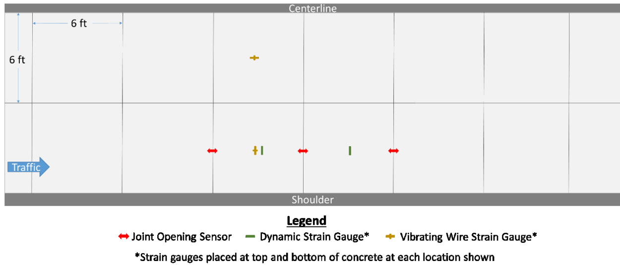
Figure 4.19 Sensor layout for FRC Cell 506.
